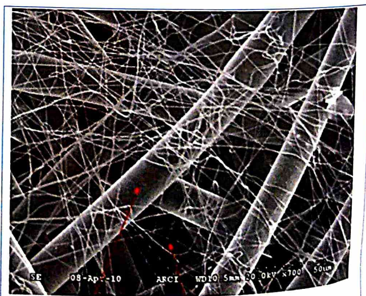
Base medium fiber Nanofibers Nanofibers covers the micron size pores of base medium and traps the fine particles.
